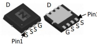
DFN3*3
